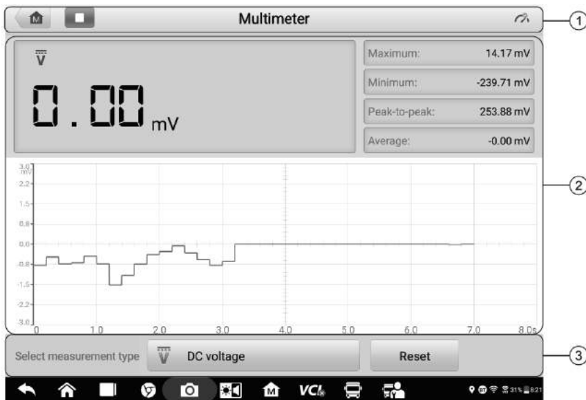
Figure 8-1 Sample Multimeter Home Screen
