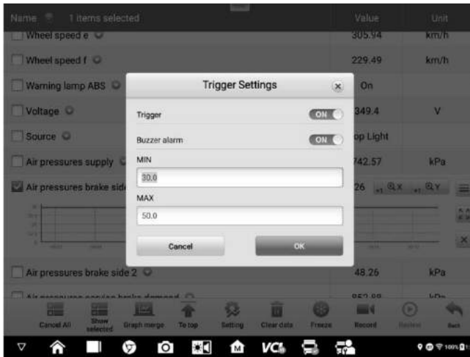
Figure 4-20 Sample Trigger Settings Screen
