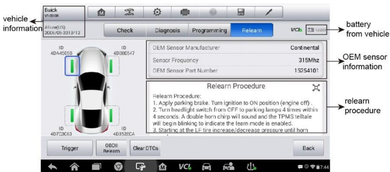
Figure 6-24 Sample Stationary Relearn Screen 1
