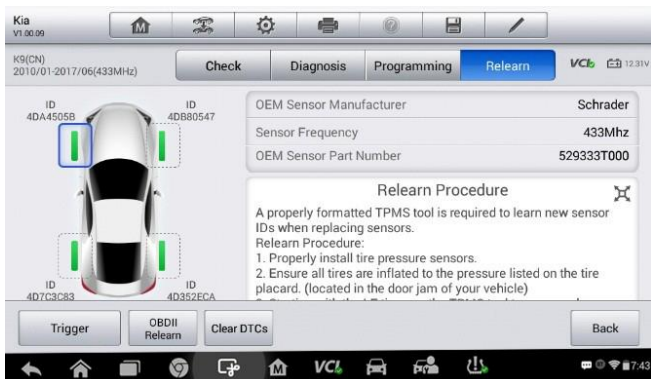
Figure 6-28 Sample OBD II Relearn Screen 1
